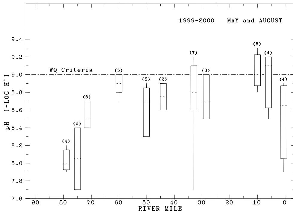
Figure 5-1. Sprague River Longitudinal pH (Box and Whiskers Plot)
